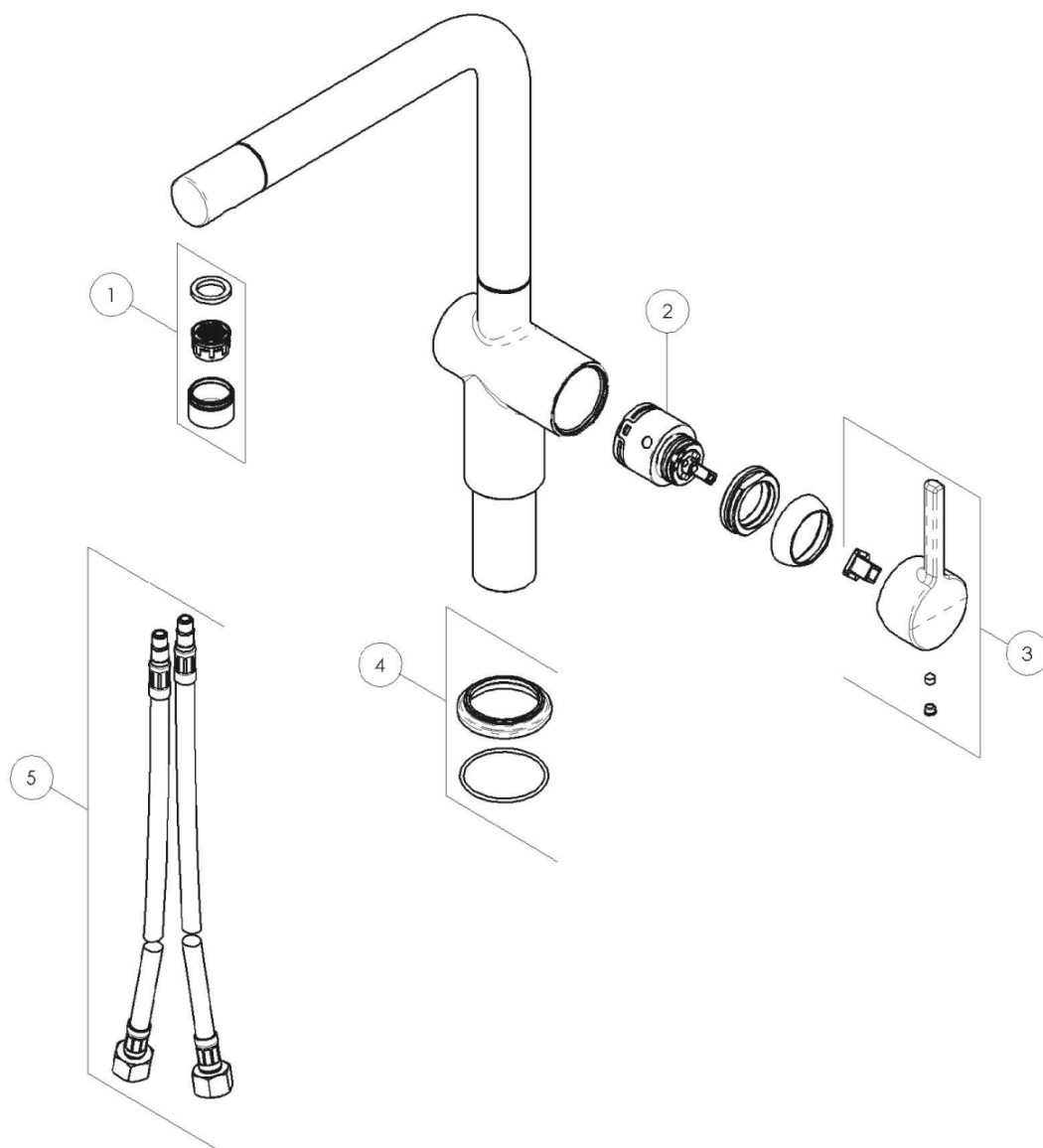
ACTIVE Swivel Spout L 115.0653.377 CHR/CO
