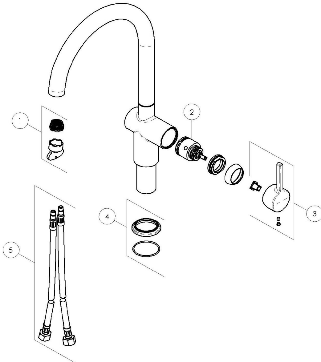
ACTIVE J Swivel Spout 115.0656.873 CHR FAJ
