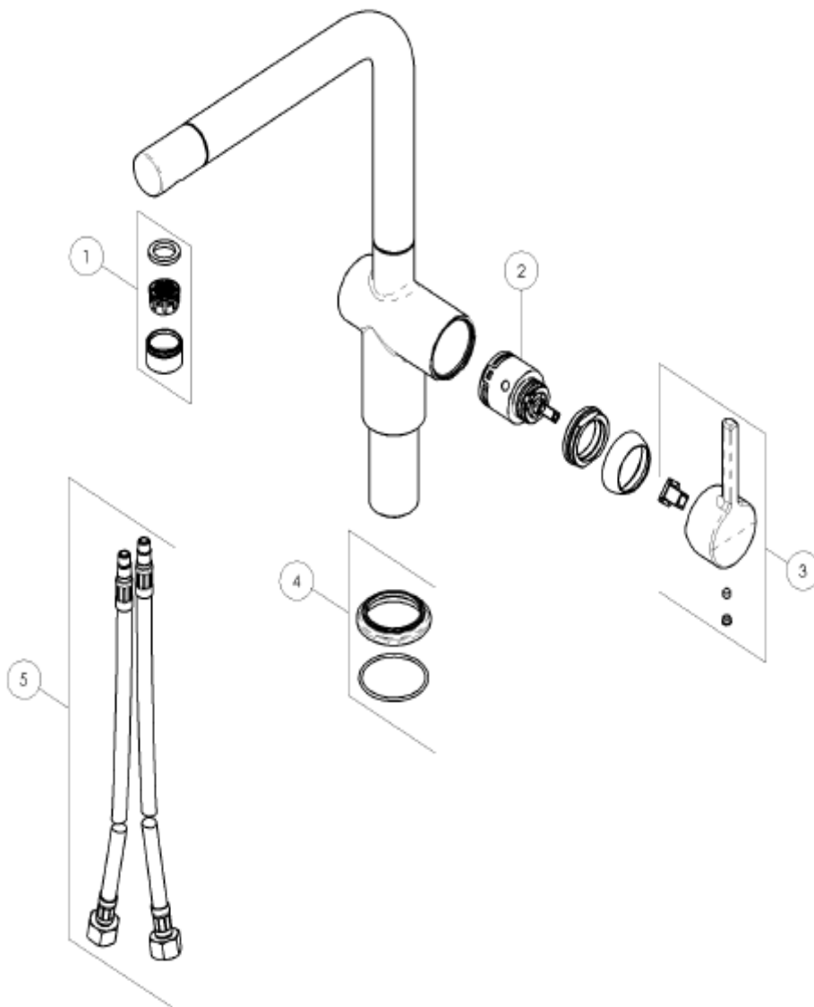
Active Swivel Spout L CHR/OA
