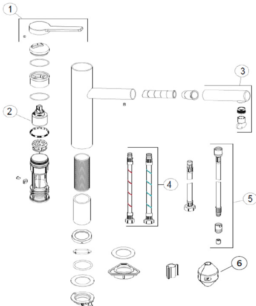
Tango Neo Pull Out Nozzle Top HP SS
